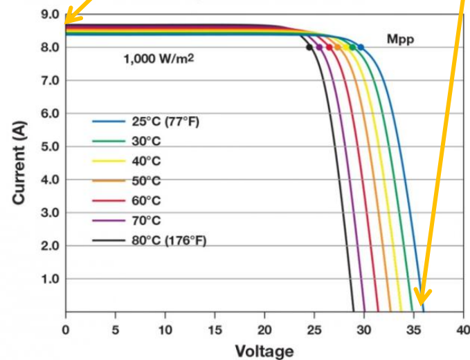
Effect of Cell Temperature on MPP
