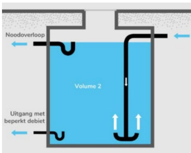
BUFFERTANK (STORMWATER)
